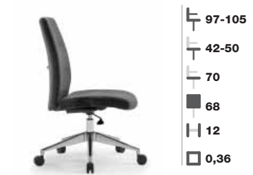
AT 8708 Direzionale, sincrono, base in alluminio Medium back executive, synchron mechanism, aluminium base
